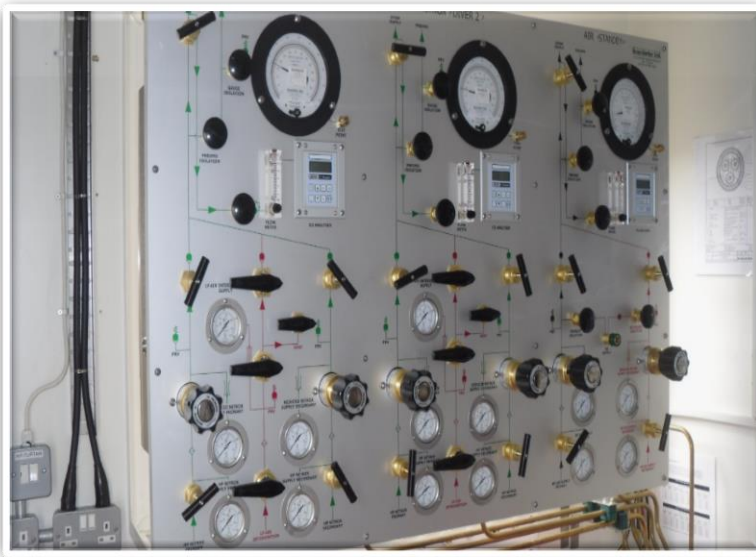
3 Diver Panel; 2 x HP Nitrox Modules (with LP Air Intervention) & 1x Standby Diver Air Module
